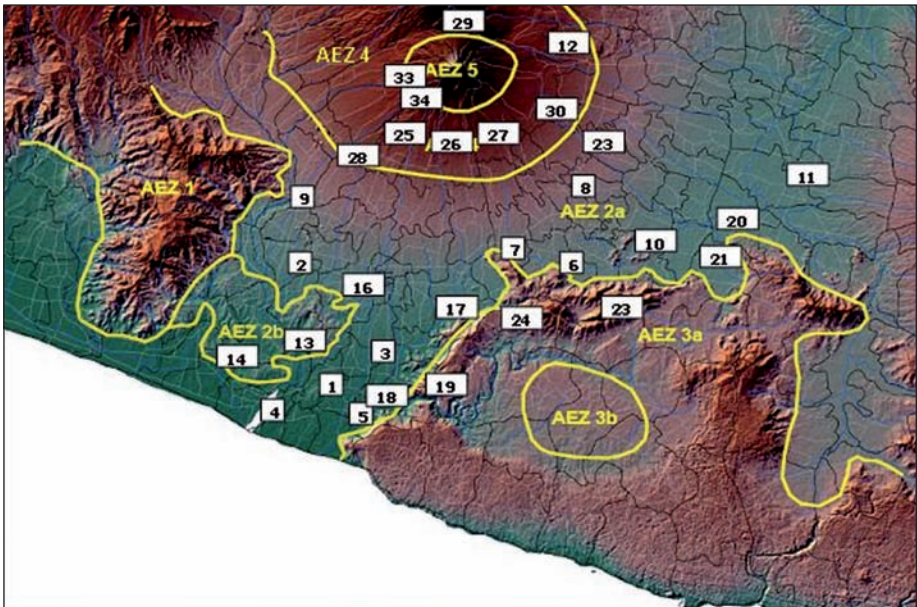
Figure 3: Yogyakarta and Central Java AEZ map
